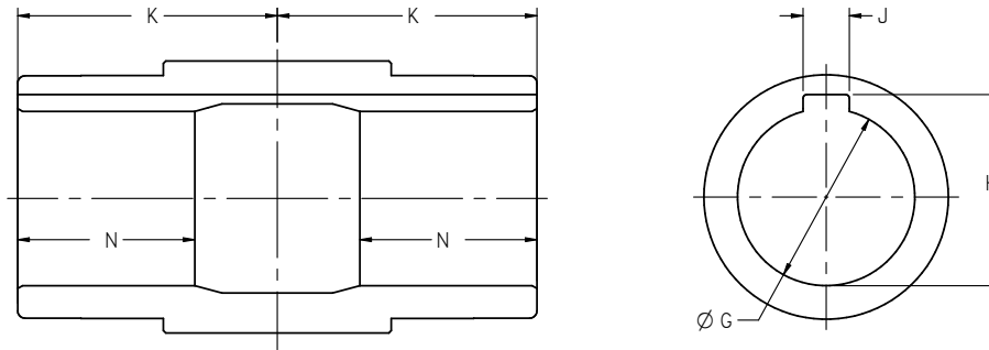
Output Bore
