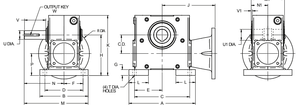
MOTORIZED
