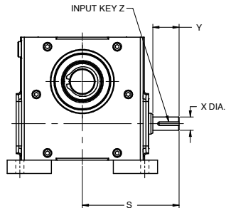
REDUCER
