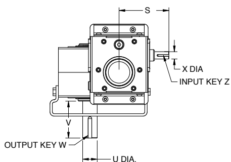
REDUCER
