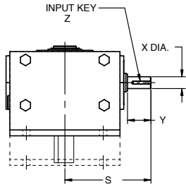
REDUCER
